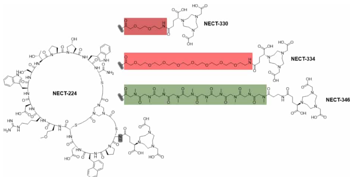
Figure 1. Structures of NECT-330, NECT-334, and NECT-346 in comparison to NECT-224.
