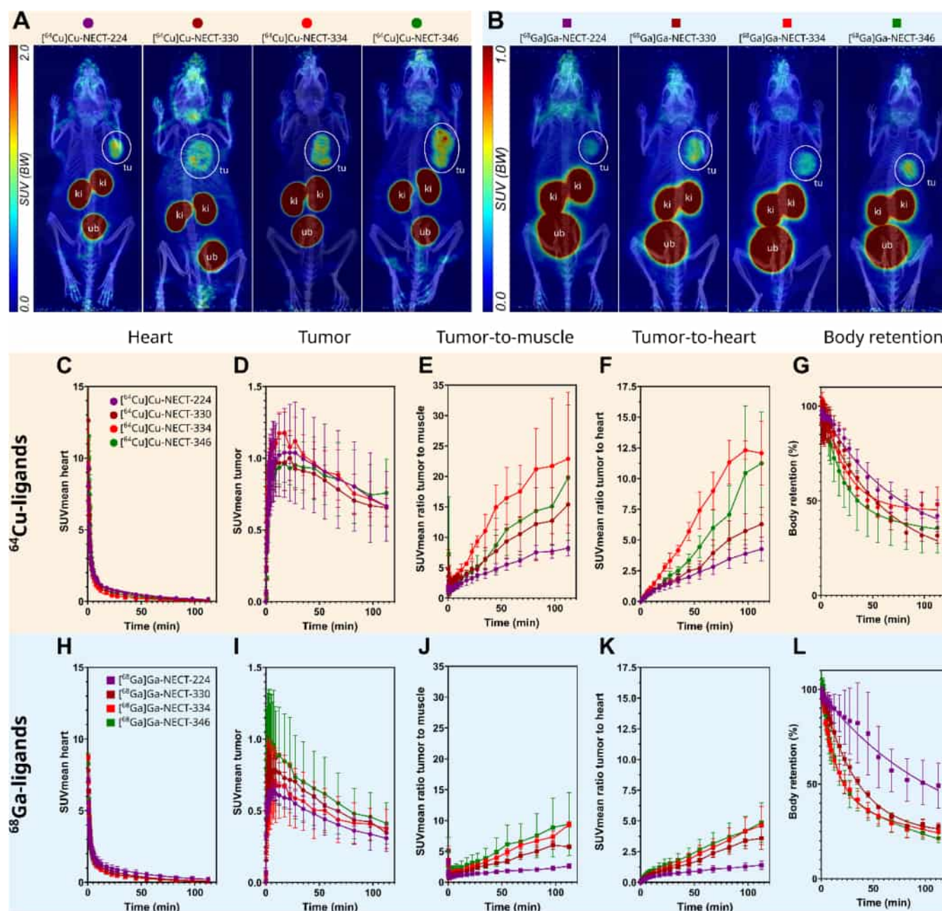
Figure 4. PET images and image-derived uptake values of the ^{64}\text{Cu} - and ^{68}\text{Ga} -labeled Nectin-4 ligands in HT-1376 tumor-bearing mice. A/B PET/CT images at 1–2 h after intravenous injection of the indicated ^{64}\text{Cu} -labeled ( A ) and ^{68}\text{Ga} -labeled ligands ( B ) in HT-1376 tumor-bearing mice. 6–9 MBq/animal (0.3–0.45 nmol/animal) were injected. Images are presented as maximum-intensity projections with a common scale (SUV 0–2 for ^{64}\text{Cu} -labeled and SUV 0–1 for ^{68}\text{Ga} -labeled ligands). Anatomical positions of the tumor (tu), kidney (ki), and urinary bladder (ub) are shown. C/D/H/I Time-activity curves (SUVmean, decay-corrected, as a function of time up to 2 h) for the blood content of the heart ( C/H ) and tumor ( D/I ) obtained from quantitative analysis of PET images are depicted for the ^{64}\text{Cu} -labeled ( C/D ) and ^{68}\text{Ga} -labeled ligands ( H/I ). E/F/J/K Time-resolved SUVmean ratios up to 2 h p.i., including tumor-to-muscle ( E/J ) and tumor-to-heart ( F/K ) for the ^{64}\text{Cu} -labeled ( E/F ) and ^{68}\text{Ga} -labeled ligands ( J/K ). G/L Time-resolved body retention in % of the initial dose up to 2 h p.i. for the ^{64}\text{Cu} -labeled ( G ) and ^{68}\text{Ga} -labeled ligands ( L ). Data points in C–L represent mean values ( \pm SD) measured in groups of HT-1376 tumor-bearing mice ( n = 6 for ^{64}\text{Cu} -Cu-NECT-224, n = 4 for ^{64}\text{Cu} -Cu-NECT-334, and ^{68}\text{Ga} -Ga-NECT-346 or n = 3 ). All data shown for ^{64}\text{Cu} -Cu-NECT-224 were previously published by us 39 and were included for reasons of comparison.
