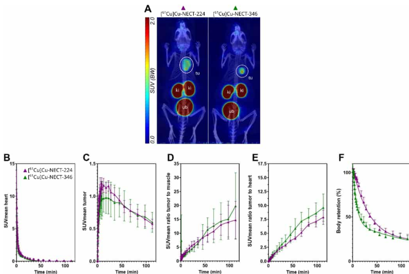
Figure 5. PET images and image-derived uptake values of ^{61}\text{Cu} -labeled NECT-224 and NECT-346 in HT-1376 tumor-bearing mice. A) PET/CT images at 1–2 h after intravenous injection of ^{61}\text{Cu} -NECT-224 and ^{61}\text{Cu} -NECT-346 in HT-1376 tumor-bearing mice. 6–9 MBq/animal (0.3–0.45 nmol/animal) were injected. Images are presented as maximum-intensity projections with a common scale. Anatomical positions of the tumor (tu), kidney (ki), and urinary bladder (ub) are shown. B/C) Time-activity curves (SUVmean, decay-corrected, as a function of time up to 2 h) for the blood content of the heart ( B ) and tumor ( C ) obtained from quantitative analysis of PET images are depicted. D/E) Time-resolved SUVmean ratios up to 2 h p.i., including tumor-to-muscle ( D ) and tumor-to-heart ( E ). F) Time-resolved body retention in % of the initial dose up to 2 h p.i. Data points in B–F represent mean values ( \pm SD) measured in groups of HT-1376 tumor-bearing mice ( n = 4 ).
