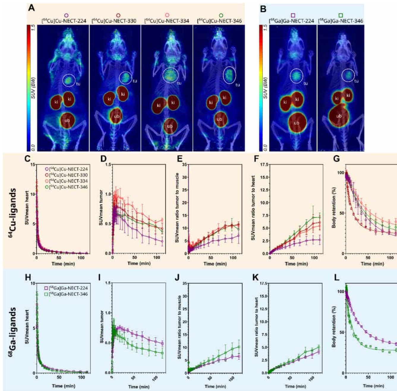
Figure 6. PET images and image-derived uptake values of the ^{64}\text{Cu} - and ^{68}\text{Ga} -labeled Nectin-4 ligands in MDA-MB-468 tumor-bearing mice. Exemplary PET/CT images of ^{64}\text{Cu} -labeled (A) and ^{68}\text{Ga} -labeled (B) ligands in MDA-MB-468 tumor-bearing mice at 1 to 2 h after intravenous injection of the indicated radiotracers. 6–9 MBq/animal (0.3–0.45 nmol/animal) were injected. All images are scaled to a maximum SUV of 1.5. C/D/H/I) Time-activity curves (SUVmean, decay-corrected, as a function of time up to 2 h) for the blood content of the heart (C/H) and of the tumor (D/I) of ^{64}\text{Cu} -labeled (C/D) and ^{68}\text{Ga} -labeled ligands (H/I), respectively, obtained from quantitative analysis of PET images. Time-resolved SUVmean ratios up to 2 h p.i., including tumor-to-muscle (E/J) and tumor-to-heart (F/K) of ^{64}\text{Cu} -labeled (E/F) and ^{68}\text{Ga} -labeled ligands (J/K), respectively. G/L) Time-resolved body retention in % of the initial dose up to 2 h p.i. Data points in C–L represent mean values ( \pm SD) of groups of three tumor-bearing mice, except for ^{68}\text{Ga} -Ga-NECT-346 which represents only two mice.
