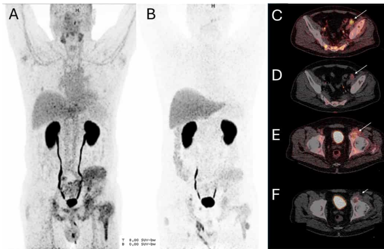
Figure 7. First-in-human application of [ ^{64}\text{Cu} ]Cu-NECT-224. A/B) Maximum-intensity projection (MIP) scaled to a maximum standardized uptake value (SUVmax) of 8, acquired in the anterior view, demonstrating the physiological distribution of [ ^{64}\text{Cu} ]Cu-NECT-224 alongside multiple tumor manifestations. Imaging was performed at 67 min (A) and 16.5 h (B) after intravenous injection of 251 MBq of [ ^{64}\text{Cu} ]Cu-NECT-224. C/D) Representative axial fused PET/CT images (scaled to an SUVmax of 8) are shown with a left external iliac lymph node metastasis indicated by a white arrow (C at 67 min and D at 16.5 h p.i.). E/F) Representative axial fused PET/CT images (scaled to an SUVmax of 8) are shown with a bone metastasis with a soft-tissue component indicated by a white arrow (E at 67 min and F at 16.5 h p.i.).
