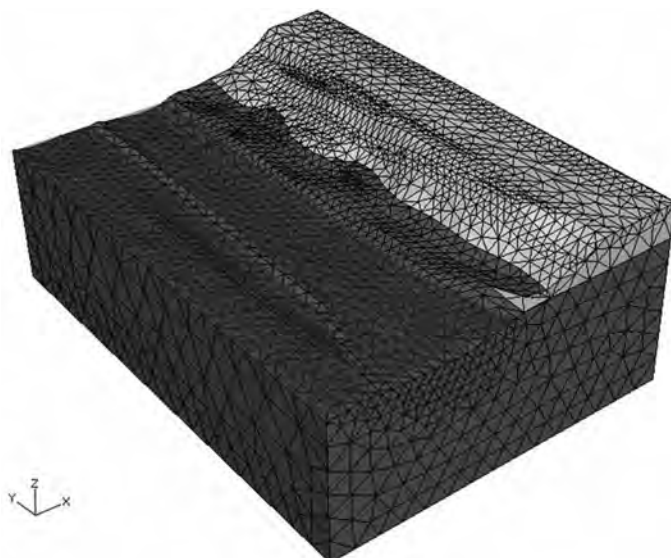
Fig. 6: FE-mesh for the wire-frame model (Fig. 5)
