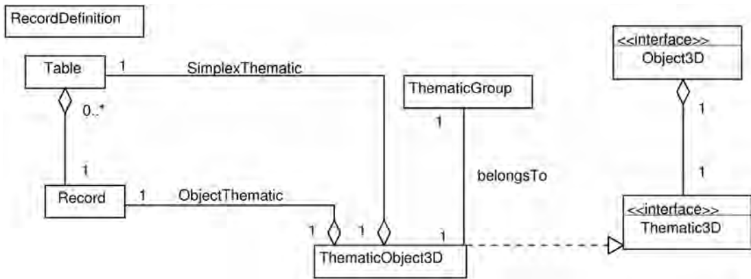
Fig. 16: Thematic model of the database objects, showed in UML notation
