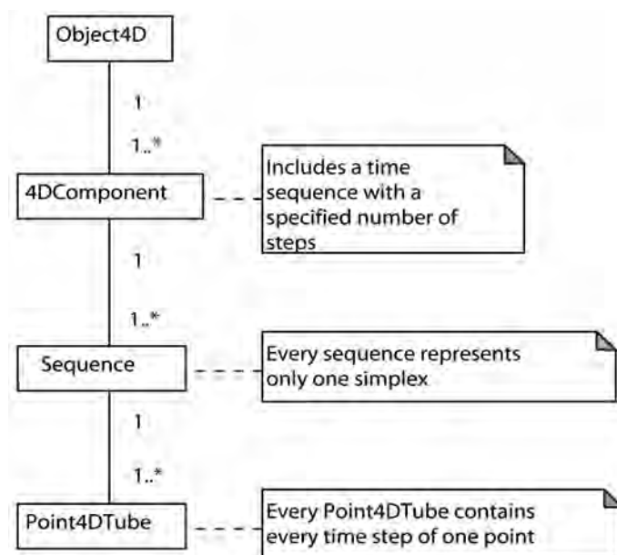
Fig. 15: Structure of 4D objects in DB4GeO
