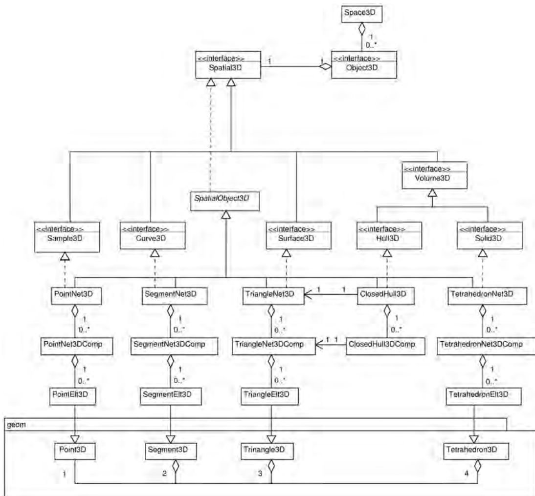
Fig. 14: Geometric model of DB4GeO in UML notation (figure from (Bär, 2007))
