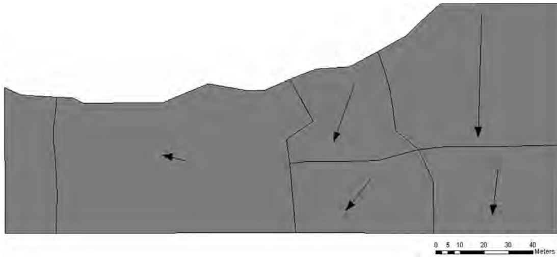
Fig. 8: Deformation vectors for different areas
