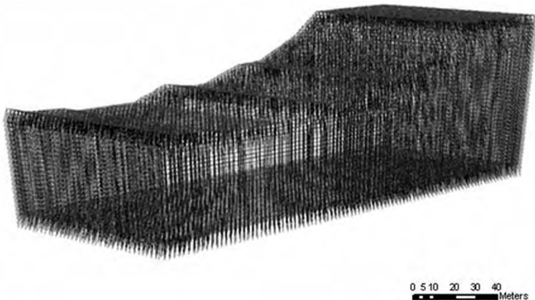
Fig. 7: Visualized deformation vectors from a 3D analysis
