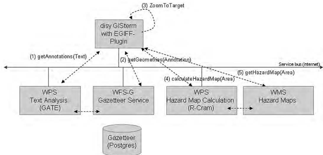
Fig. 19: EGIF service based integration of components
