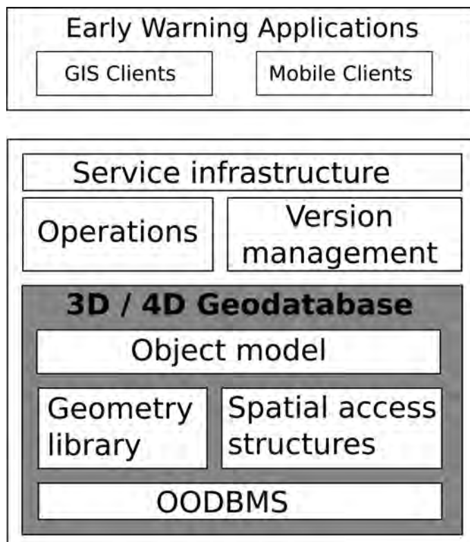
Fig. 13: System architecture of DB4GeO
