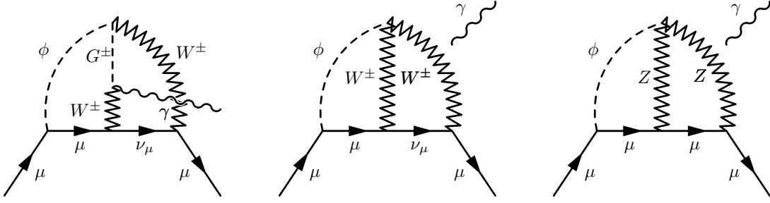
Figure 4: Two-loop bosonic three boson contribution included within GM2Calc, where \phi = h, H, A . In the middle and right diagrams the photon can couple to either of the vector bosons. Also in the right diagram the neutral Higgs can swap its position with one of the Z bosons.
