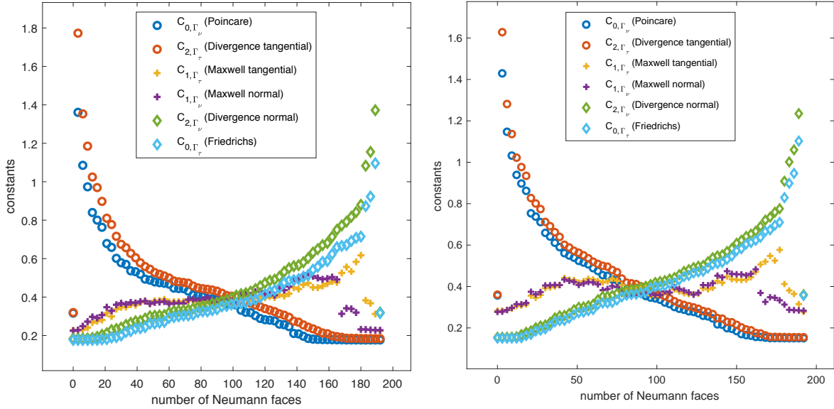
FIGURE 7. Constants computed for the level 1 meshes of unit cube domain (left) and of the Fichera corner domain (right) - monotonicity test for a monotone increasing sequence of Neumann faces \Gamma_\nu .
