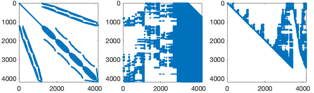
FIGURE 9. An example of a positive semidefinite matrix K \in \mathbb{R}^{4184 \times 4184} (left) taken as a K^N matrix from level 2 mesh discretization of the unit cube domain and matrices \tilde{Q} (middle) and \tilde{R} (right) from the QR decomposition (23). The number of last zero rows of \tilde{R} is 728 and it determines the dimension of the kernel of K . Therefore, the dimension of the range of K is 3456.
