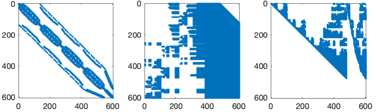
FIGURE 8. An example of a positive semidefinite matrix K \in \mathbb{R}^{604 \times 604} (left) taken as a K^N matrix from level 1 mesh discretization of the unit cube domain and matrices \tilde{Q} (middle) and \tilde{R} (right) from the QR decomposition (23). The number of last zero rows of \tilde{R} is 124 and it determines the dimension of the kernel of K . Therefore, the dimension of the range of K is 480.
