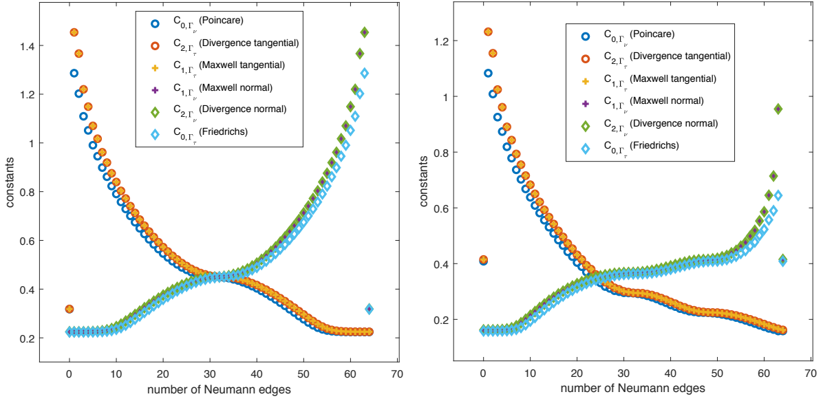
FIGURE 6. Constants computed for the level 3 meshes of the unit square domain (left) and of the L-shape domain (right) - monotonicity test for a monotone increasing sequence of Neumann edges \Gamma_\nu .
