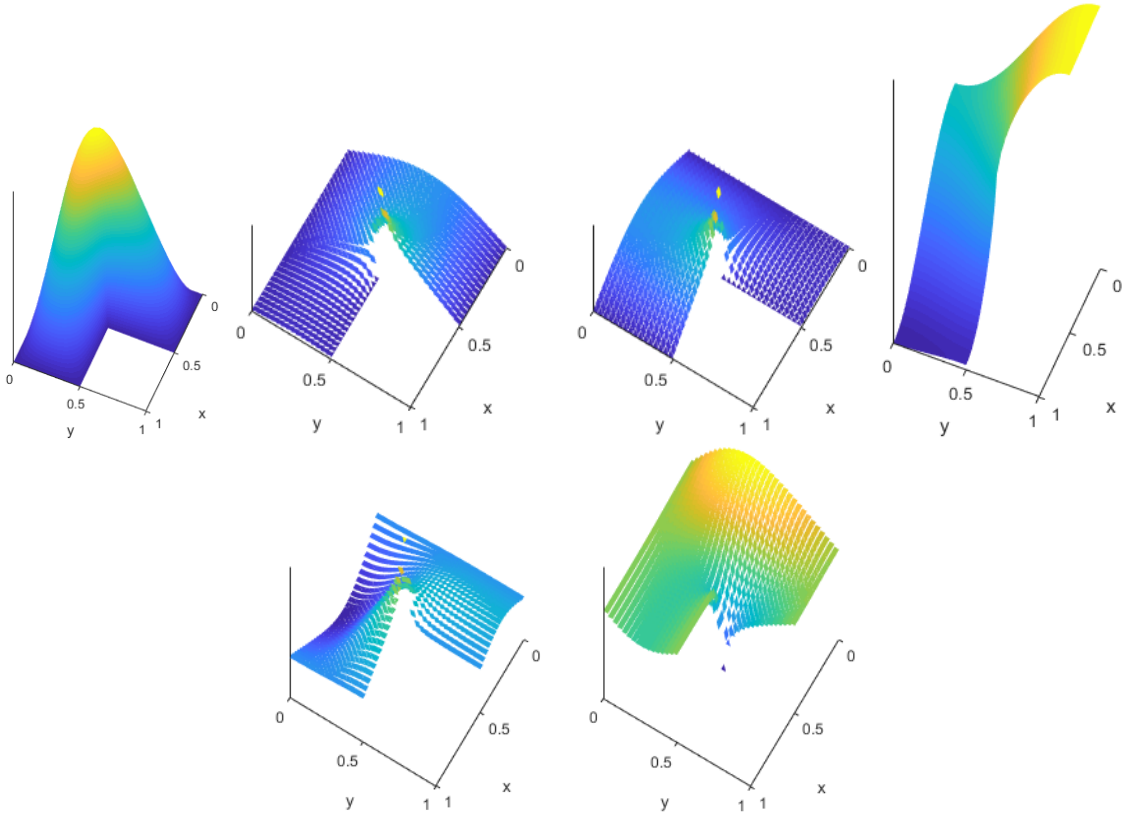
FIGURE 10. Eigenfunctions - Friedrichs (top left), Poincaré (bottom left), tangential Maxwell (top middle and right), normal Maxwell (bottom middle and right) - for the L-shape domain with full boundary conditions.
