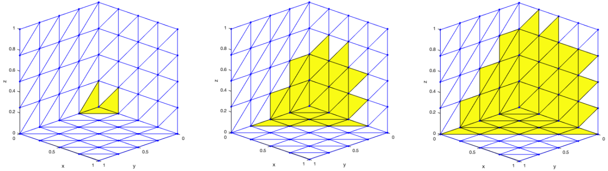
FIGURE 5. Elements of a monotone increasing sequence of Neumann faces \Gamma_\nu with 3 (left), 27 (middle) and 51 (right) Neumann faces marked in yellow. A full boundary \Gamma of the considered level 1 mesh of the unit cube domain consists of 192 faces.
