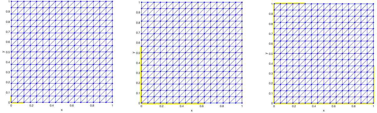
FIGURE 4. Elements of a monotone increasing sequence of Neumann edges \Gamma_\nu with 3 (left), 7 (middle) and 19 (right) Neumann edges marked in yellow. A full boundary \Gamma of the considered level 2 mesh of the unit square domain consists of 32 edges.
